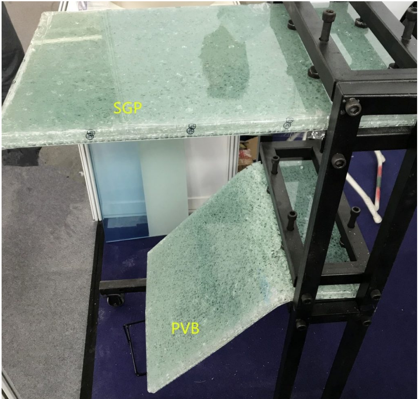
sgp vs pvb breakage
