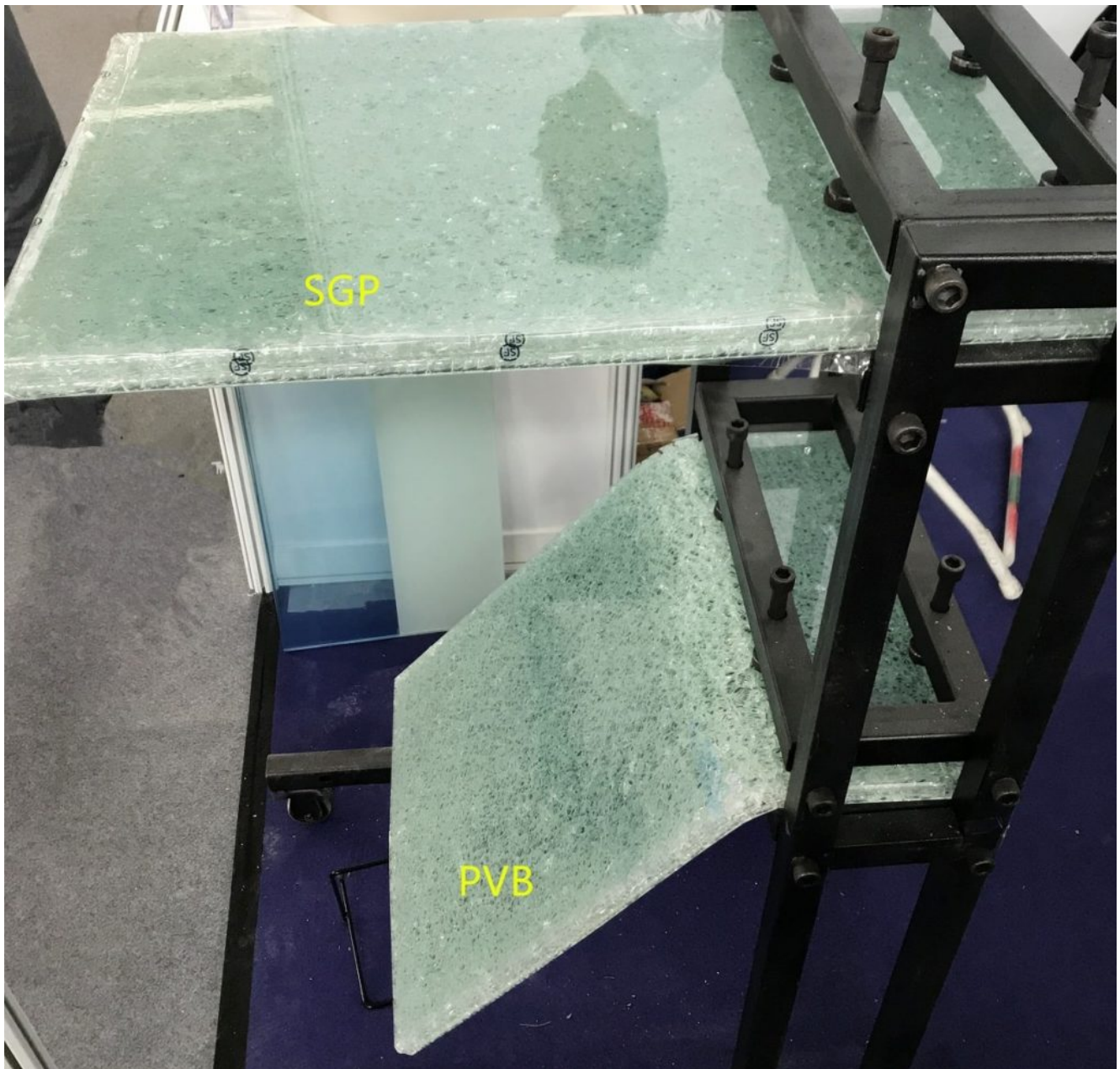
sgp vs pvb bruch
