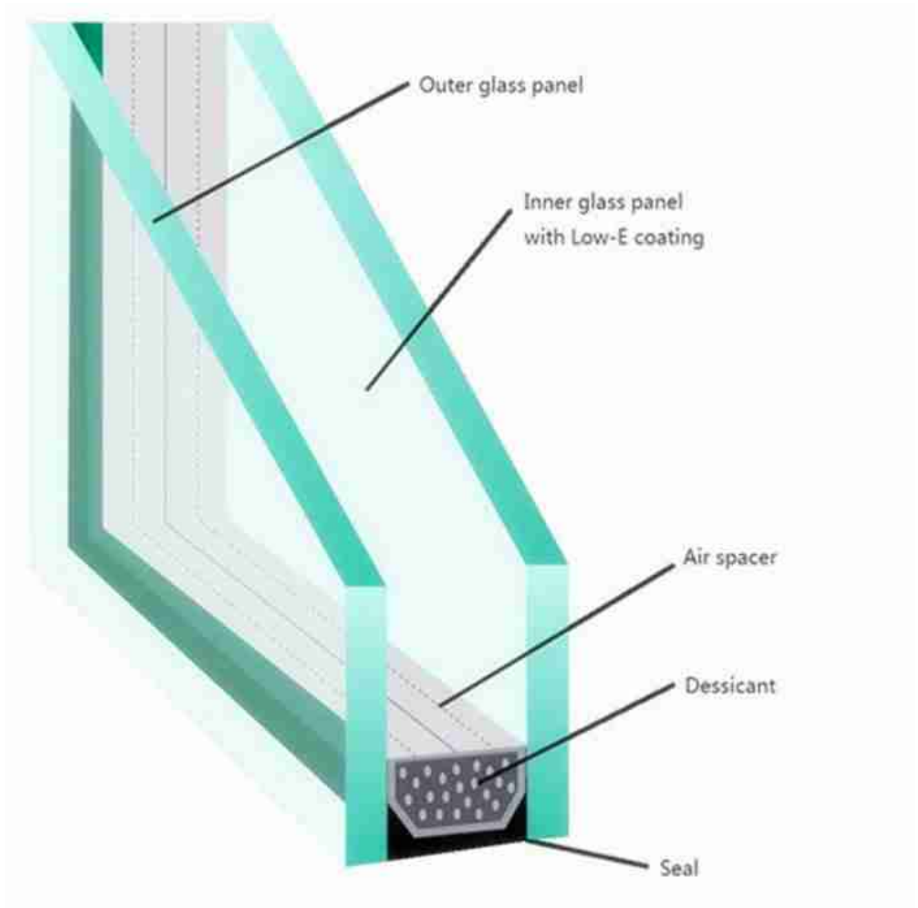
dgu glass structures
