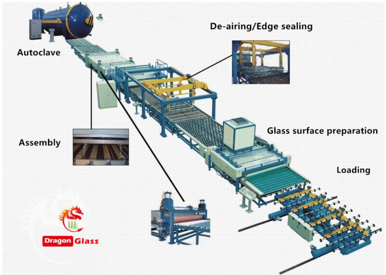
Gradient color laminated glass production line
